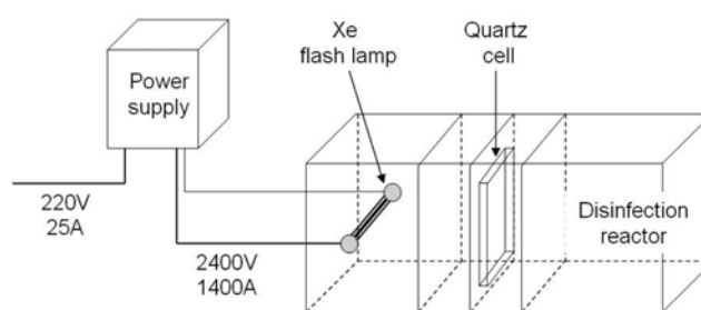
Fig. 1. A schematic of the pulsed UV irradiation system used in this study.
