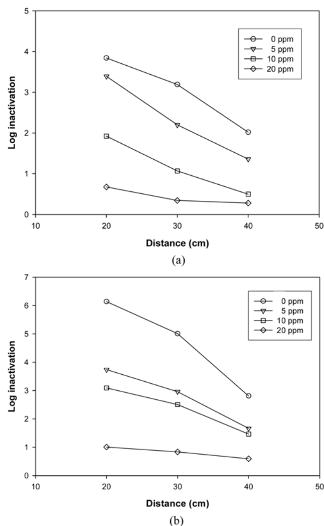
Fig. 5. Effect of humic acids on E. coli inactivation by pulsed UV irradiation. (a) 3 sec and (b) 5 sec of irradiation time.
