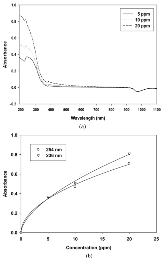
Fig. 6. (a) The absorbance spectrum of the humic acid mixture at different concentrations and (b) the extent of UV absorption by humic acids at 254 nm and 236 nm.
