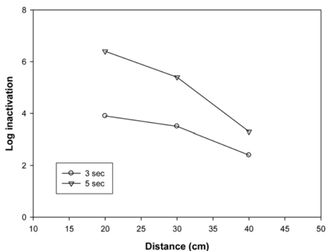
Fig. 3. Inactivation at different distances and irradiation times.
